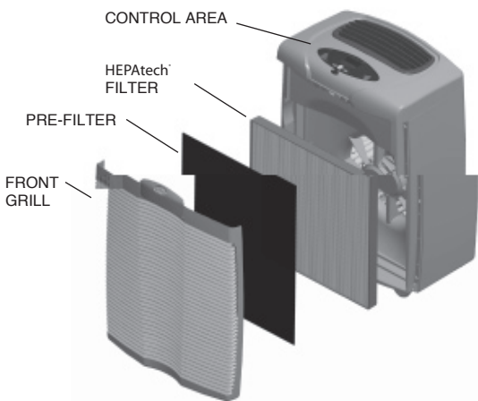
Fig. 2 - Air Purifier Components
